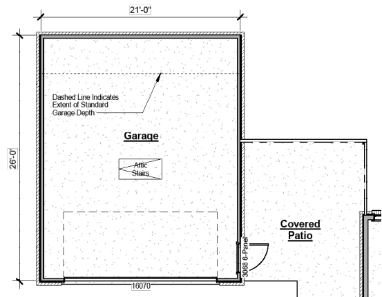
4ft Garage Extension
