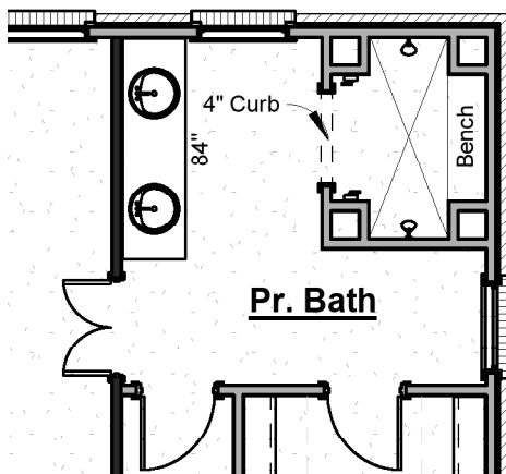
Primary Bath with Grotto Shower
