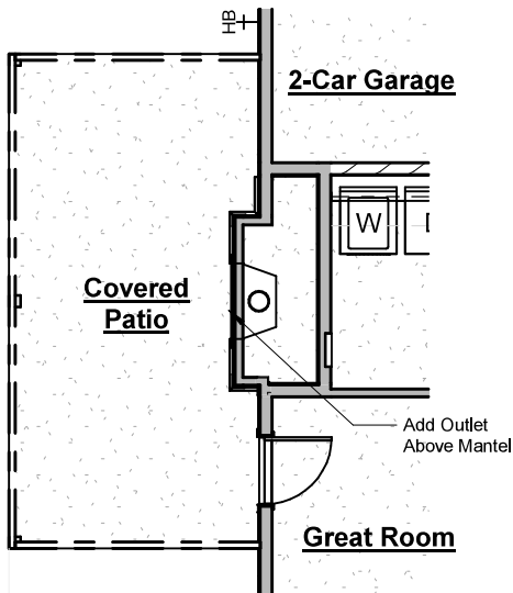
Outdoor Gas Log Fireplace
