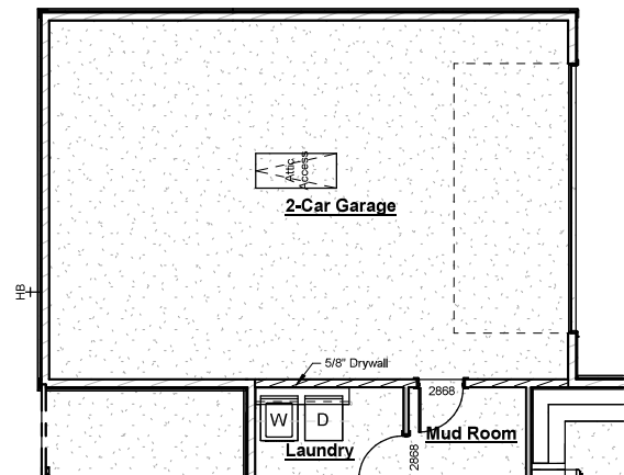
2-Car Garage Extension
