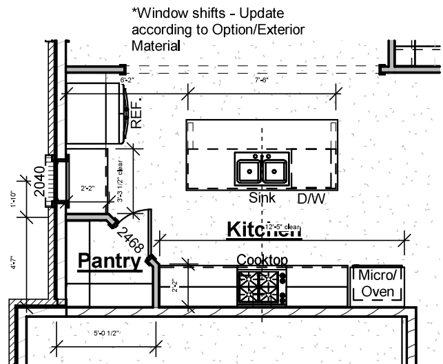
Corner Pantry
