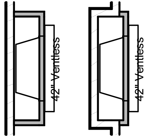
42" Firebox Option
