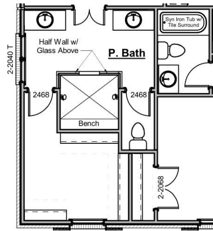
Primary Bath with Grotto Shower
