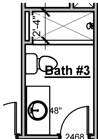
Bath #3 Tile Shower
