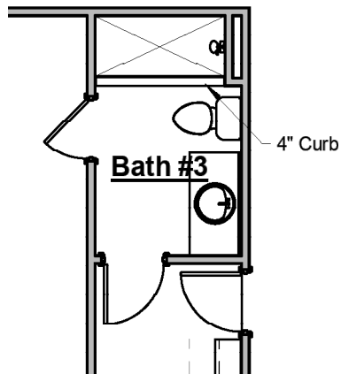
2nd Floor - 4th Bedroom & 3rd Bath with Guest Bath Tile Shower
