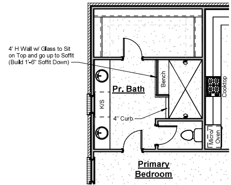
Primary Bath Spa Shower
