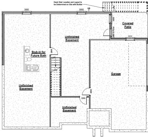
Unfinished Basement with Basement Garage
