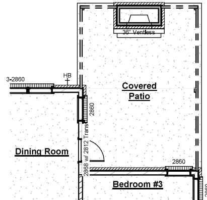
Extension with Outdoor Gas Log Fireplace
