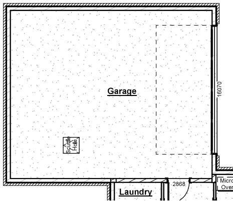
4ft Garage Extension
