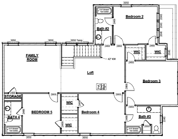
Family Room with 5th Bed & 4th Bath Option
