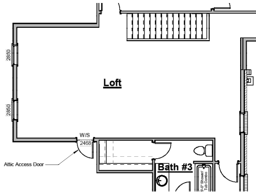
Extended Loft
