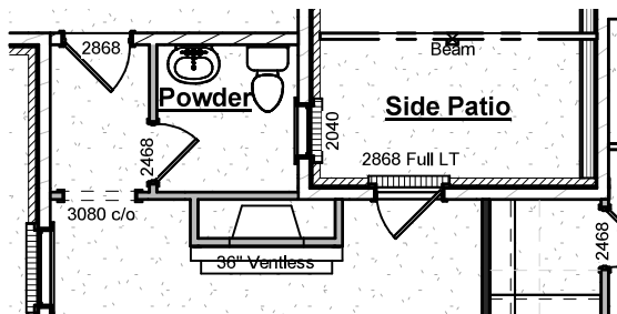
Powder Room
