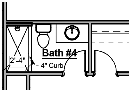
Bath 4 Tile Shower
