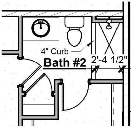
Bath 2 Tile Shower
