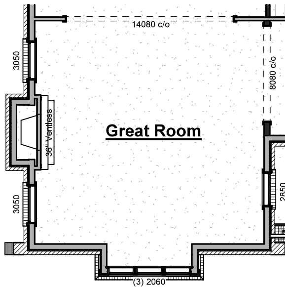
Great Room Fireplace Bump-Out
