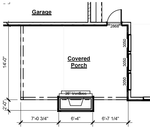
Covered Patio Extension with Side Fireplace
