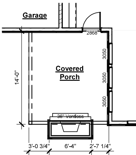
Covered Patio Standard with Side Fireplace
