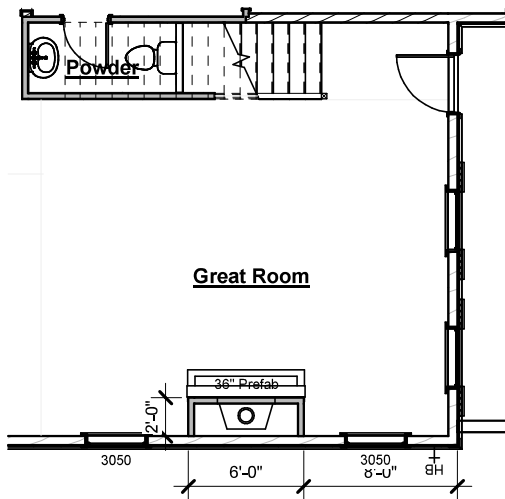
Great Room Fireplace Bump-In
