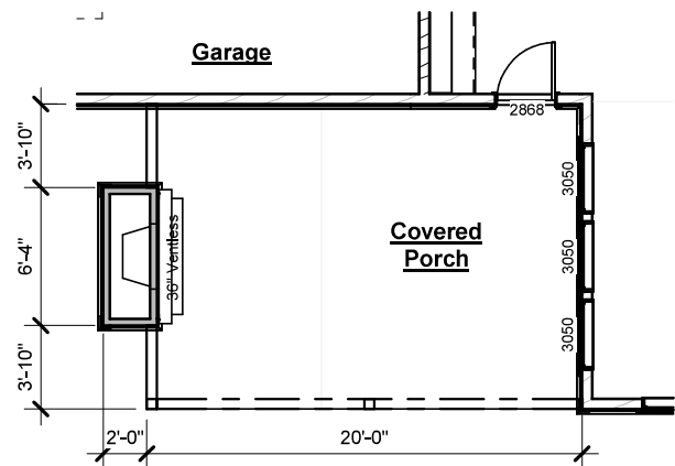
Covered Patio Extension with Rear Fireplace
