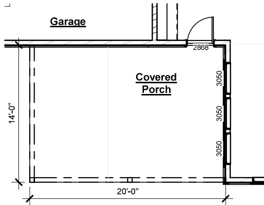
Covered Patio Extension
