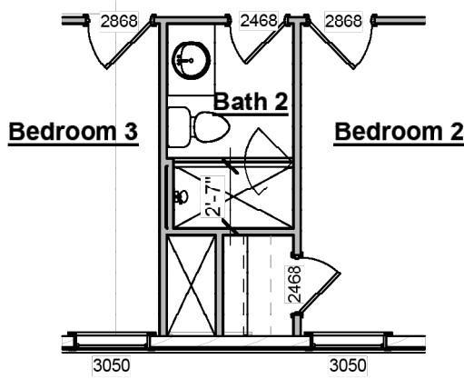
Bath 2 Tile Shower
