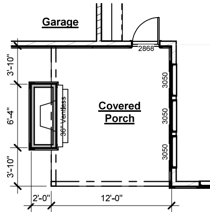
Covered Patio Standard with Rear Fireplace
