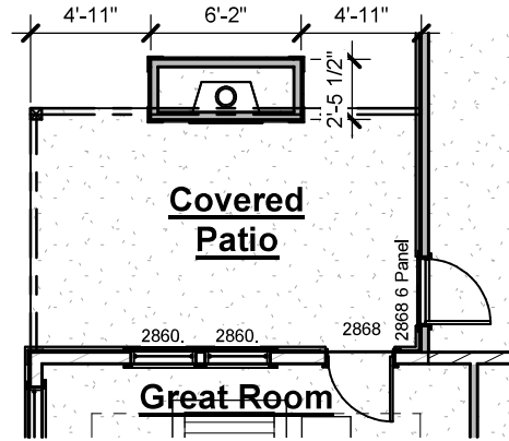
Outdoor Gas Log Fireplace with Cedar Mantel
