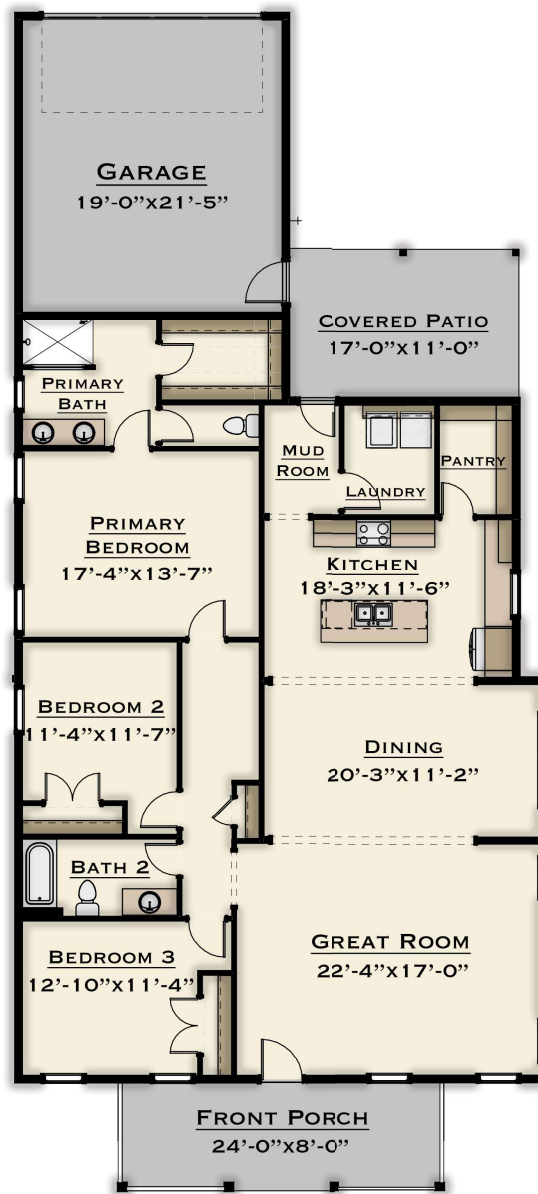
Main Level - D
