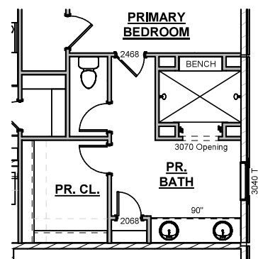
Primary Bath with Grotto Shower
