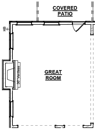
Great Room Fireplace Bump-Out
