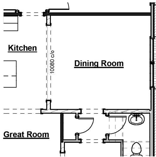
Cased Opening at Kitchen/Dining Room
