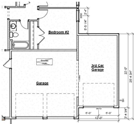
3rd Car Garage
