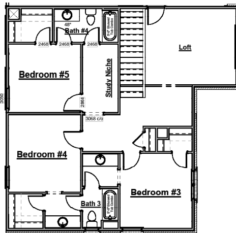
5th Bedroom with Bath 4 Option
