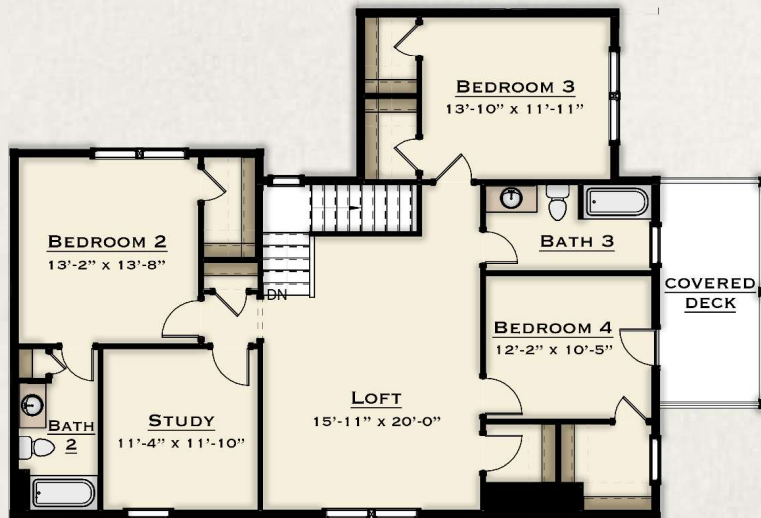
Second Floor B
