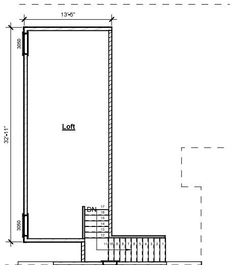
2nd Floor Loft Option
