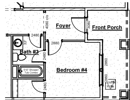
4th Bedroom & 3rd Bath
