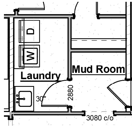
Laundry Room Sink
