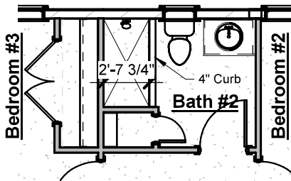
Bath #2 Tile Shower
