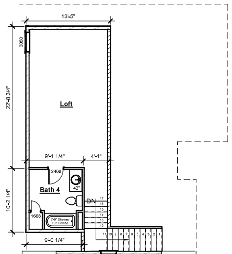
2nd Floor Loft Option w/ Bath
