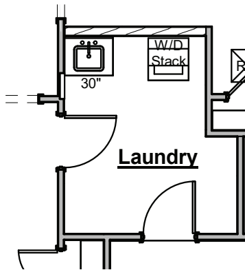
Laundry Room Sink Option
