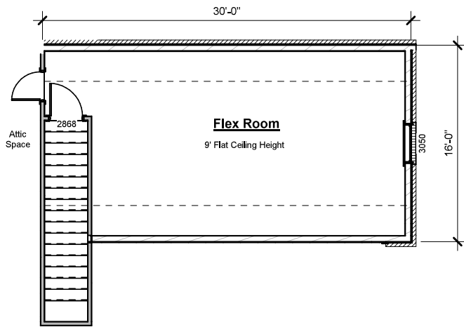
Finished 2nd Floor
