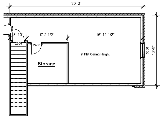
Finished 2nd Floor with Storage
