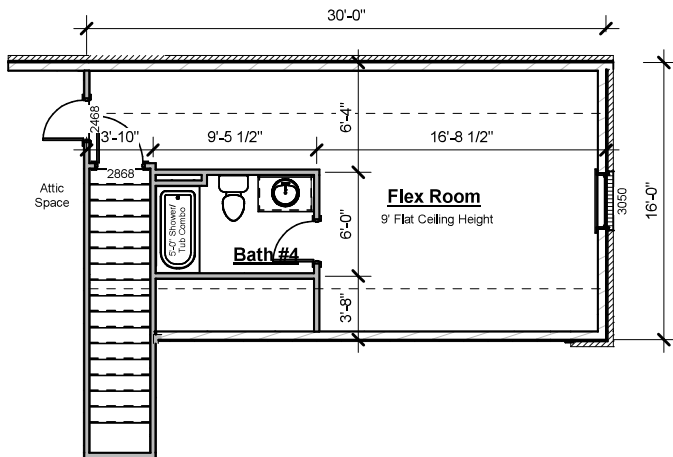
Finished 2nd Floor & Bath
