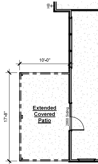
Covered Patio Extension
