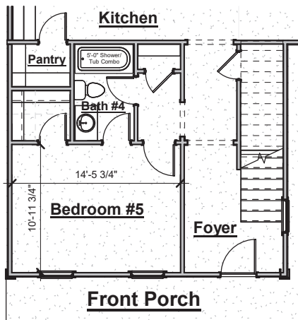
Bedroom #5 with Bath #4
