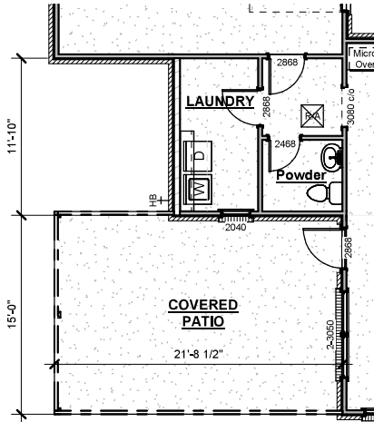
Covered Patio Extension
