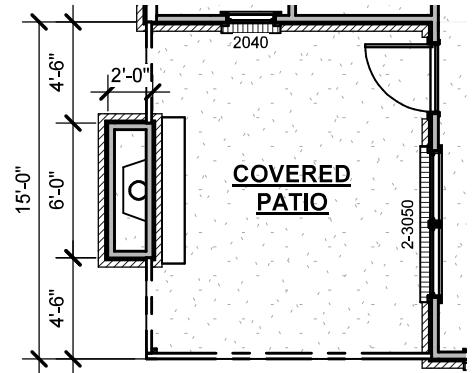
Outdoor Gas Log Fireplace
