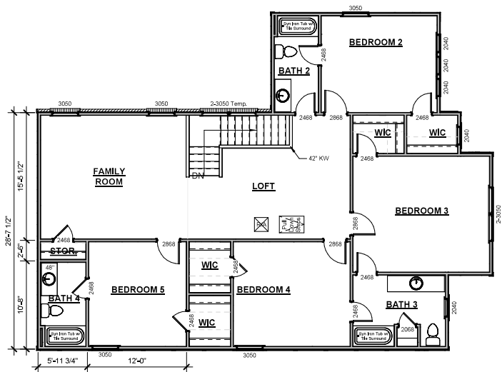
Family Room with 5th Bed & 4th Bath Option
