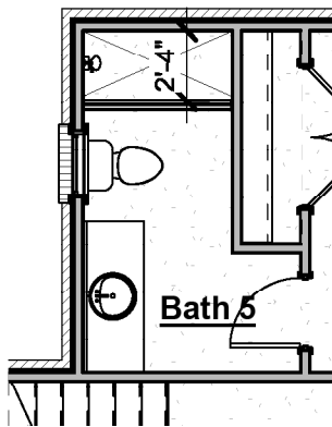
Bath 5 Tile Shower
