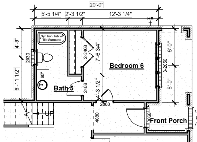
3rd Car Garage Conversion - 6th Bed & 5th Bath
