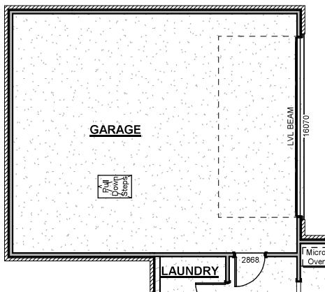
4ft Garage Extension
