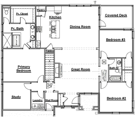
1st Floor Plan for Basement Plan
