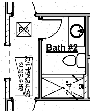
Bath #2 Tile Shower
