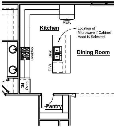
Chef's Kitchen with Double Oven
