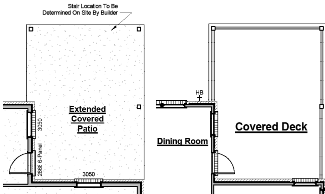
Basement Covered Patio Extension
