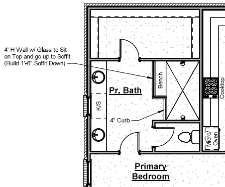
Primary Bath Spa Shower
