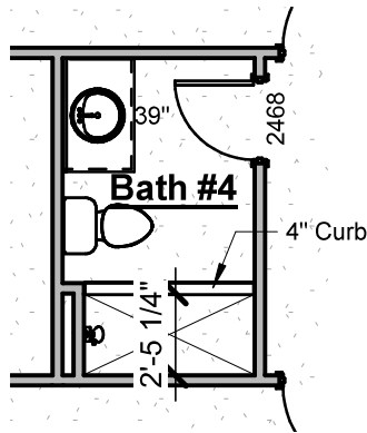
Bath #4 Tile Shower
