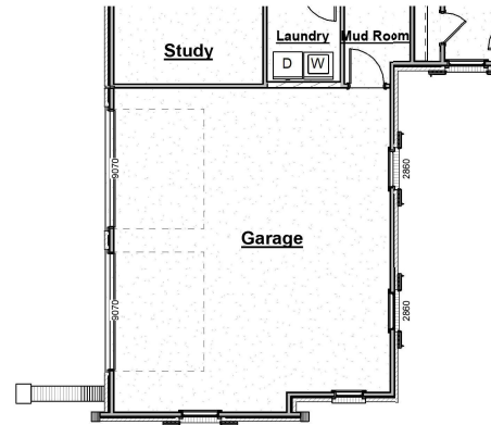
Side Load Garage
