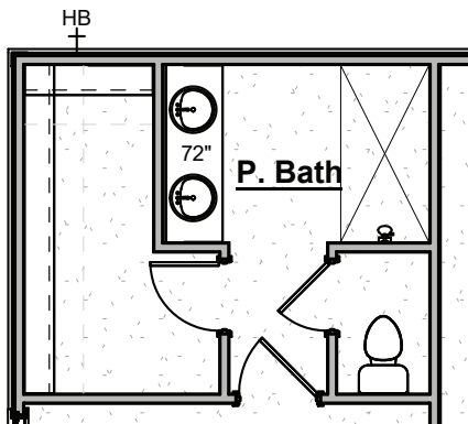
Primary Bath Double Bowl Vanity
