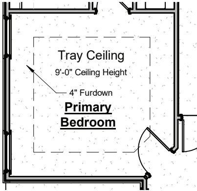
Primary Bedroom Tray Ceiling Option
