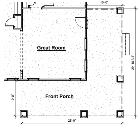
Wrap Around Front Porch
