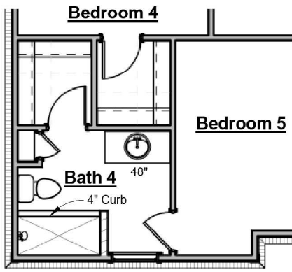
Bath 4 Tile Shower
