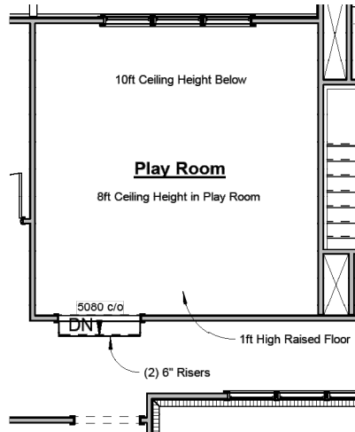
2nd Floor - Play Room
