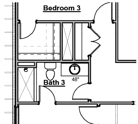
Bath 3 Tile Shower
