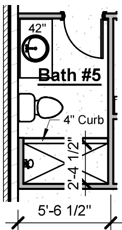
Bath 5 Tile Shower
